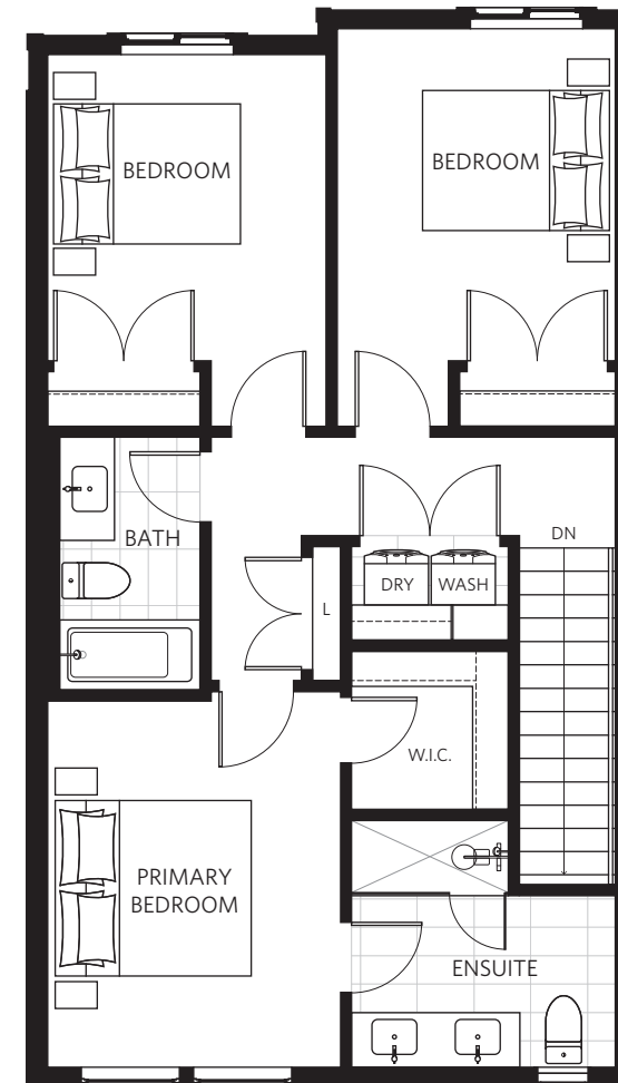
UPPER LEVEL
